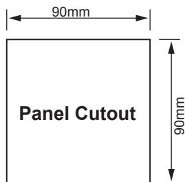
Figure 6: Case Dimensions
